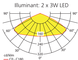
Ceiling mounting
