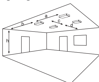
Ceiling mounting
