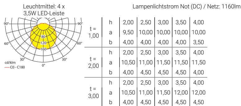
Wandmontage
